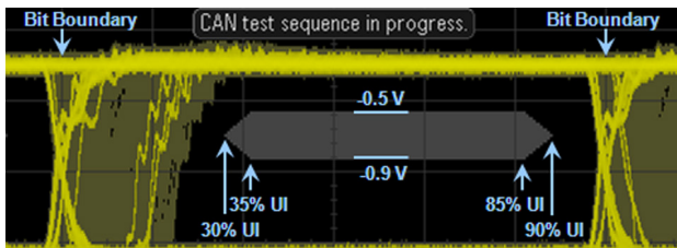
Figure 8: Pass/Fail mask for a 10 meter network operating at 500 kbps.
